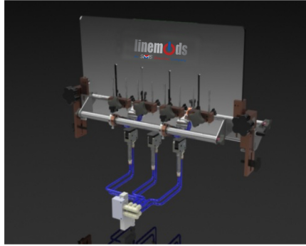
Flip Plate (Tipper Plate)
